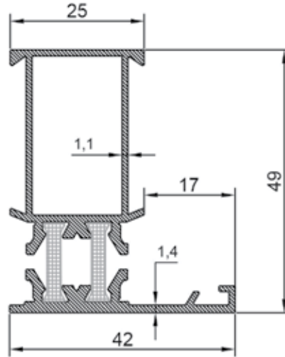
ER 2350-2353 0,870 kg/m Dar Kasa Profili / Narrow Casing Profile I_x = 8,498 \text{ cm}^4 I_y = 3,096 \text{ cm}^4
